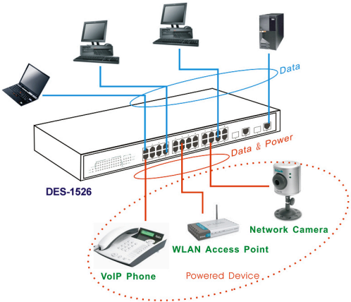
Figure 4. Connecting Network Cables
