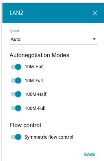
Figure 106. The window for changing the settings of the router's port.
